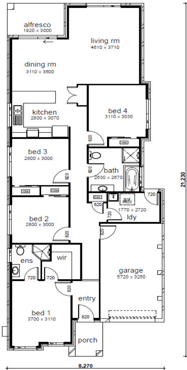
Floor Plan
